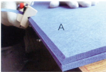
◆ 折疊吸音板，給切割面“A”做45°倒角 Chamfer 45° bevel edge for side “A” by chamfering tool.
