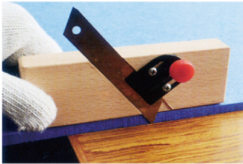
◆ 調節推刀，刀片略高於吸音板 Adjust the height of the knife.
